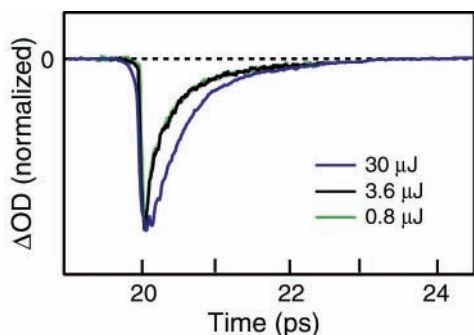
Figure 3. Ultrafast spectral relaxation dynamics of the hydrated electron ( e_{\text{eq}} ). The relaxation dynamics are independent of the timing of the control pulse. Previous spectroscopic results have demonstrated excitation of e_{\text{eq}} at 800 nm with weak excitation pulses involves a one-photon excitation, which has been assigned to the s \rightarrow p transition based on a comparison to theory and simulation. 4,5,10,11,18,22,23 After the initial absorption bleach (negative signal) because of e_{\text{eq}} depopulation, the one-photon excited p state relaxes to repopulate e_{\text{eq}} within a few picoseconds (see the 0.8 and 3.6 \mu\text{J} curves). At higher pulse energy (30 \mu\text{J} ), a previously observed two-photon sequential excitation channel is accessed resulting in slower relaxation dynamics. Because the two-photon channel occurs at an energy at which simulations predict a conduction band, the two-photon prepared state has been assigned to the conduction band from s \rightarrow p \rightarrow \text{CB} sequence. 18
