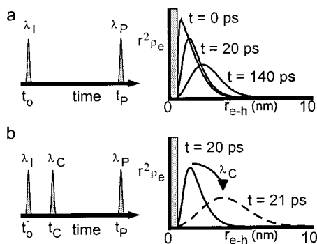
Figure 1. Schematic illustration of femtosecond laser based control of the spatial distribution and geminate recombination of the hydrated electron ( e_{\text{eq}} ). The sequence consists of an ionization ( \lambda_I ), control ( \lambda_C ), and probe ( \lambda_P ) pulse. In Figure 1a, the ionization pulse produces an initial distribution of excess electrons surrounding the hole which evolves via diffusion and e_{\text{eq}} /hole geminate recombination. In Figure 1b, an additional control pulse spatially redistributes the population of electron far from the hole suppressing the geminate recombination process. The shaded region represents the encounter region where the electron recombines with the hole. The probability distribution function used to describe the initial distribution of e_{\text{eq}} /hole separation is defined as \rho_e(r_{e-h}) = (2\pi\sigma_1^2)^{-3/2} \exp[-r_{e-h}^2/2\sigma_1^2] , where the average e_{\text{eq}} /hole separation, \bar{r}_{e-h} , is related to \sigma_1 by \bar{r}_{e-h} = 2\sqrt{2}\sigma_1/\sqrt{\pi} . The probability distribution function for the migration length of the conduction band electron is defined as \rho(l_m) = (2\pi\sigma_2^2)^{-3/2} \exp[-l_m^2/2\sigma_2^2] . The average migration length, \bar{l}_m , is related to \sigma_2 by \bar{l}_m = 2\sqrt{2}\sigma_2/\sqrt{\pi} .
